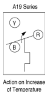
Figure 1: A19 Series terminal arrangement for Single-Pole, Double-Throw (SPDT)
