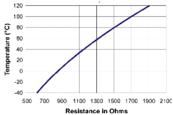
Figure 11: Resistance Scale for Celsius Temperatures
