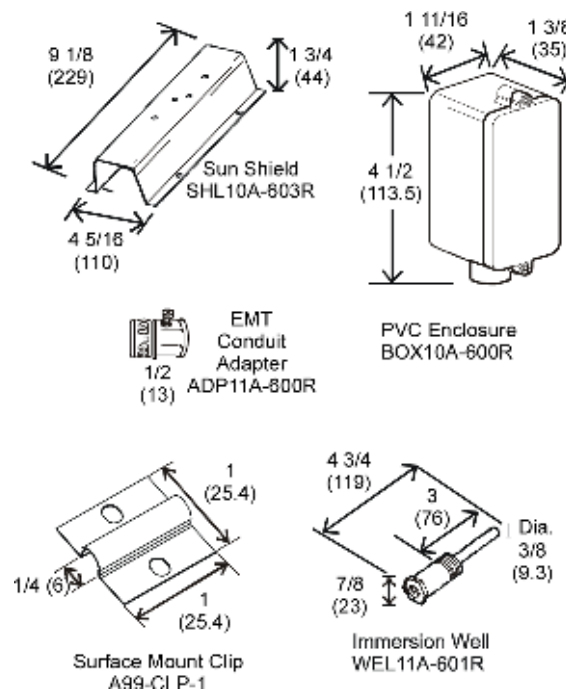
Figure 6: Available Accessories, in. (mm)
