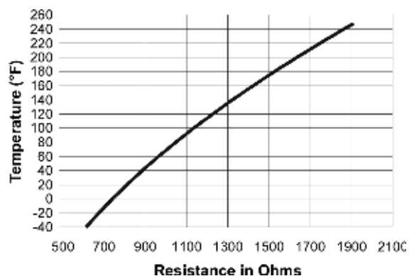
Figure 10: Resistance Scale for Fahrenheit Temperatures
