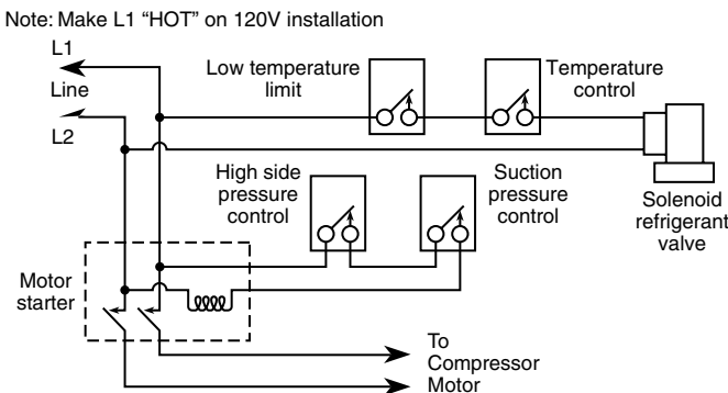
Circuit showing temperature control to open and close refrigerant valve. Suction pressure control starts and stops compressor through motor starter.
